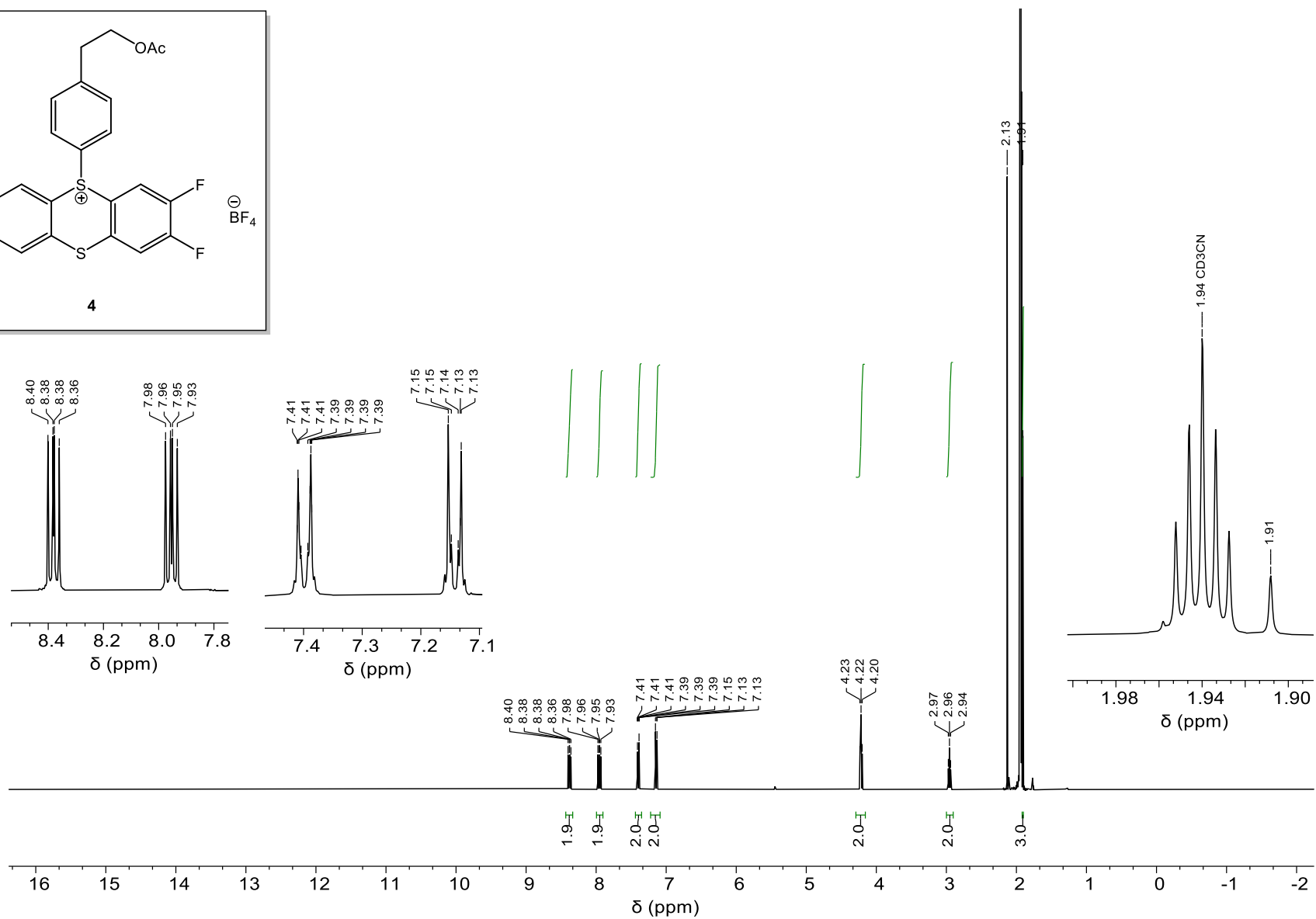
1 H NMR (400 MHz, CD 3 CN) of 2-Phenethyl acetate derived tetrafluorothianthrenium salt (4).
